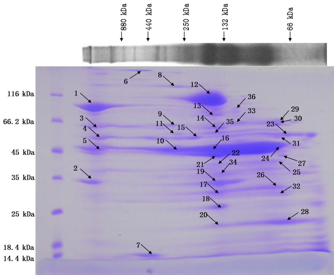
Figure 1 Coomassie blue-stained 2D BN/SDS-PAGE separation of membrane protein complexes of C. thermocellum . Approximately 40 \mu g of protein was loaded in the first dimensional BN-PAGE lane. Sizes of molecular mass markers are indicated on the top of BN-PAGE gel and at the left of the SDS gel. The slice of first dimensional BN-PAGE separation gel was placed on top of the second dimensional SDS-PAGE gel and resolved. Protein spots picked for mass spectrometry analysis are marked by arrows and numbered.
