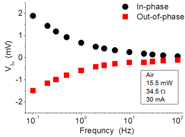
Figure S7. The in-phase and out-of-phase V_{3\omega} voltage amplitudes as a function of frequency for air.
