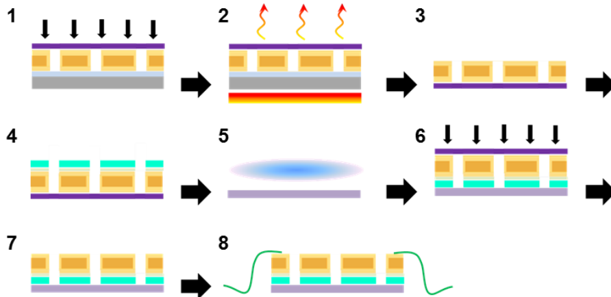
Figure S3. Fabrication procedure (part 2). (c)1. Petri dish preparation, 2. Silicone mixing and spincoating, and 3. Gentle detachment after complete curing. (d) 1. Attachment of water-soluble tape, 2. Heating, 3. Quick detachment of the tape (pattern pickup), 4. E-beam deposition of Ti/SiO 2 , 5. UV exposure, 6. Pattern transfer, 7. Tape dissolving in water, and 8. Bonding of a flexible electrical cable.
