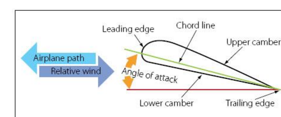
Figure 3-57. Wing terminology.
