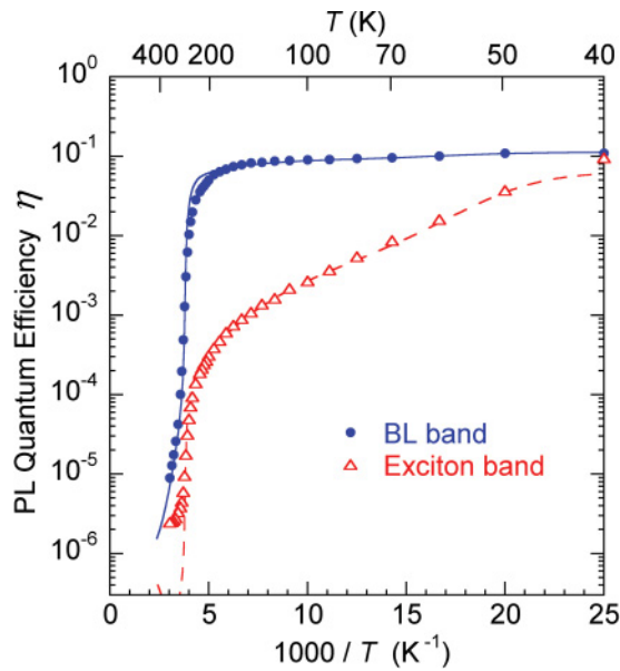
FIG. 8. (Color online) Temperature dependence of the quantum efficiency of the BL band (filled circles) and exciton band (empty triangles) for sample s451 with P_{\text{exc}} = 10 \text{ W/cm}^2 . The solid blue curve is calculated using Eqs. (7)–(12) with N_A = 4.6 \times 10^{17} , N_S = 2.7 \times 10^{17} , N_D = 1.6 \times 10^{17} (all in \text{cm}^{-3} ); C_{pS} = 2.5 \times 10^{-6} , C_{DA} = 4 \times 10^{-12} (all in \text{cm}^3/\text{s} ); and G = 1.6 \times 10^{24} \text{ cm}^{-3}\text{s}^{-1} . Other parameters are the same as for Fig. 6. The dashed red curve is calculated for the exciton emission quenching by using Eq. (29) with E_x = 33 \text{ meV} , \tau_x = \mathcal{K}T^{3/2} with \mathcal{K} = 1.3 \times 10^{-12} \text{ s K}^{-3/2} , N_{cv} = 3.4 \times 10^{14} T^{3/2} \text{ cm}^{-3} , C_x = 10^{-4} \text{ cm}^3/\text{s} , and with n and p calculated with the same parameters as for the solid blue curve.
