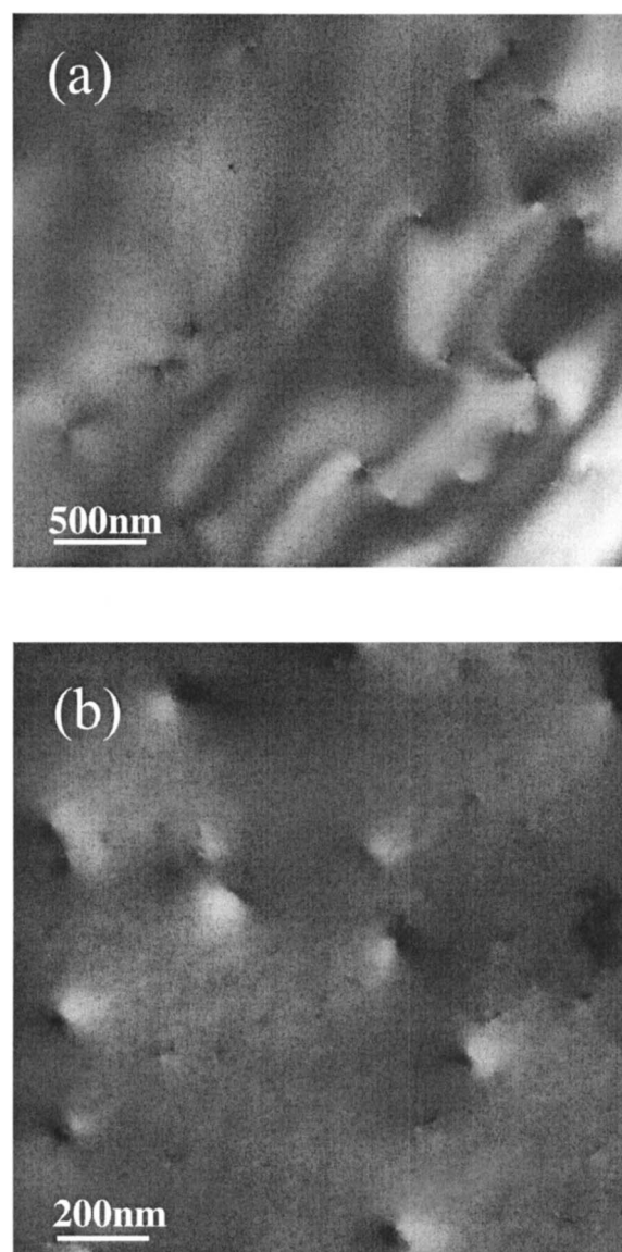
FIG. 6. Plan-view TEM image of (a) CVD 489 and (b) control GaN taken at [0001] zone axis showing edge-component dislocations.
