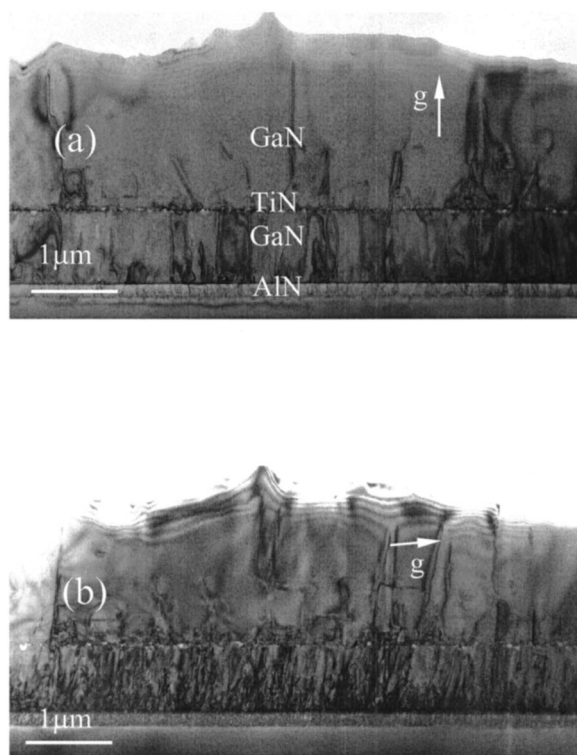
FIG. 5. Cross-sectional TEM images of CVD489 taken with (a) g=0002 to show screw or mixed dislocations and (b) g=1120 to show edge or mixed dislocations. Images of (a) and (b) come from almost the same areas.
