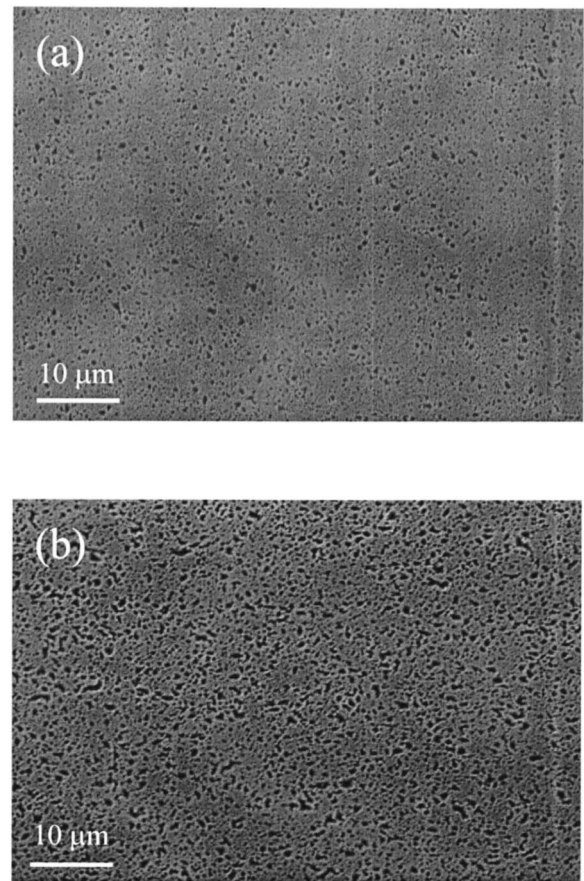
FIG. 1. SEM image of TiN networks on (a) CVD481, annealing for 10 min and (b) CVD489, annealing for 20 min.
