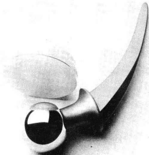
Fig. 4—The Müller total hip with a 32 mm femoral head of cobalt chrome alloy and a high density polyethylene acetabulum.
