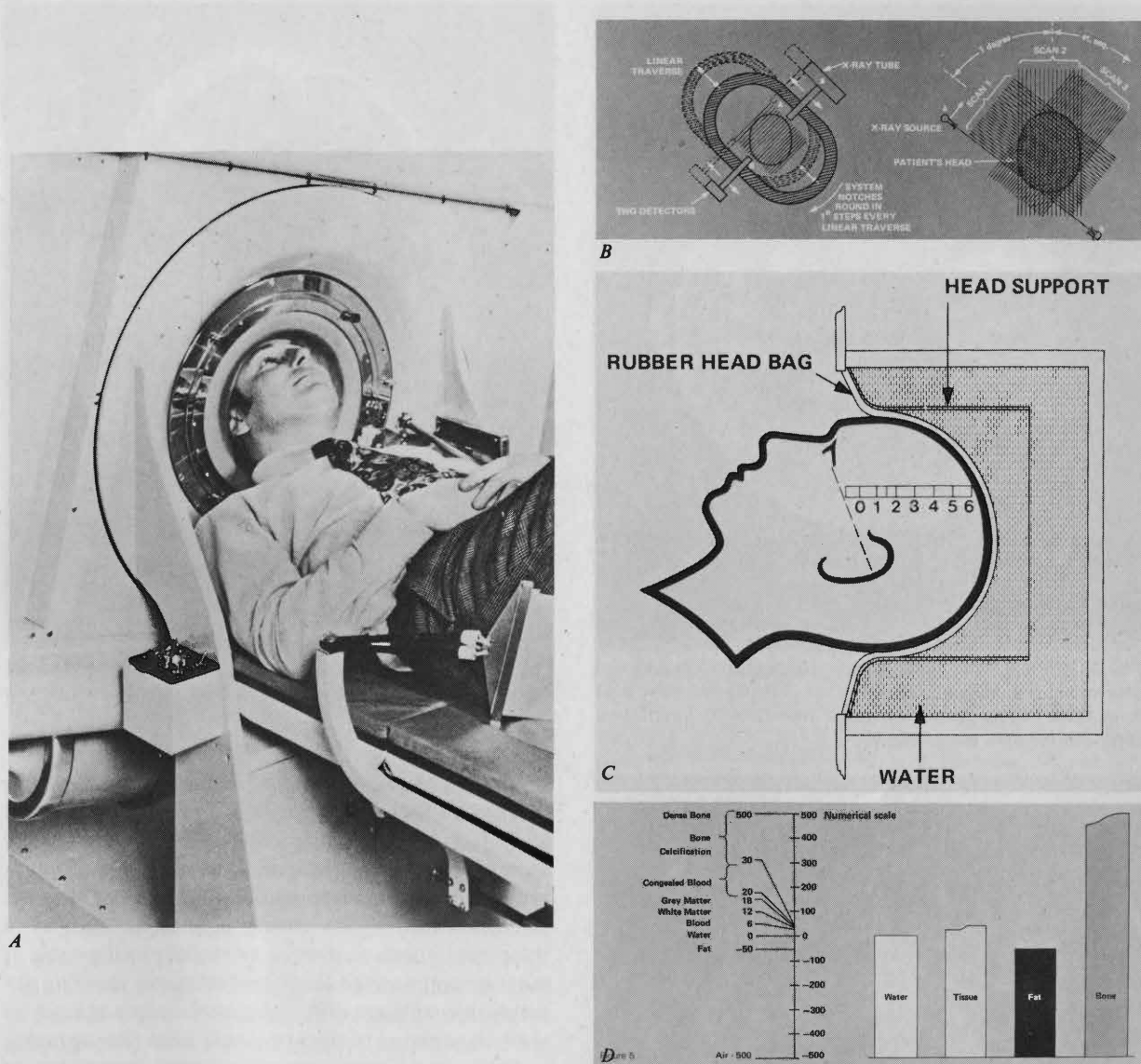
Fig. 3—A. The EMI scanner. B. Rotation sequence of scanning unit. C. Patient positioned for tomograms to include orbits and posterior fossa. D. Arbitrary scale of absorption values with air as -500 and water as 0.
