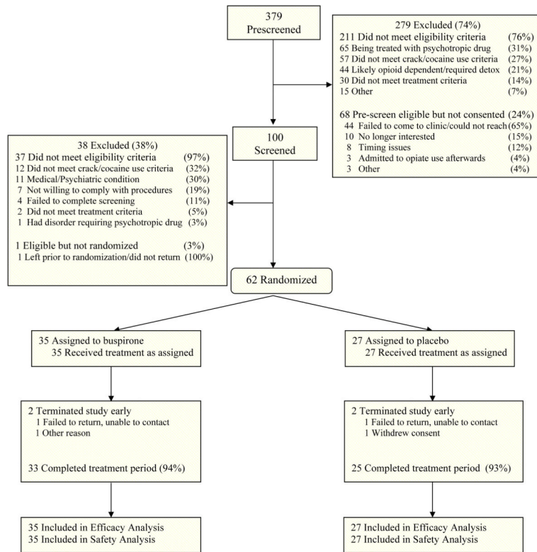
Figure 1. Participant Disposition
