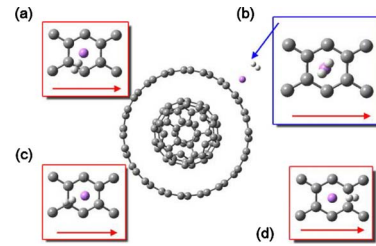
FIG. 3. (Color online) Optimized structure of H_2 on Li coated (10, 10) nanotube containing C_{60} molecule inside (nanopeapod structure). Upper right (b) blue structure is an enlarged local top view of center geometry, where hydrogen molecule is on top of Li atom with its H-H bond tangential to the CNT surface. Red arrows indicate tube axis. The other three lowest energy structures of hydrogen binding are shown in red frame, (a) with H-H bond normal to CNT surface and on top of C-C bond along the zigzag direction, (c) with H-H bond normal to CNT surface and on top of C atom, and (d) with H-H bond normal to CNT surface and on top of C-C bond along the armchair direction.
