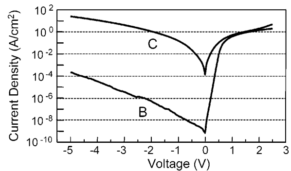
FIG. 4. I-V spectra taken on samples B and C using 75 \mu\text{m} diameter, Ni/Au Schottky contacts. Sample B indicates a field emission or thermionic field emission mechanism for forward bias, and a hopping mechanism at reverse bias. Sample C is best fit using a Frenkel-Poole mechanism for both reverse and forward bias.
