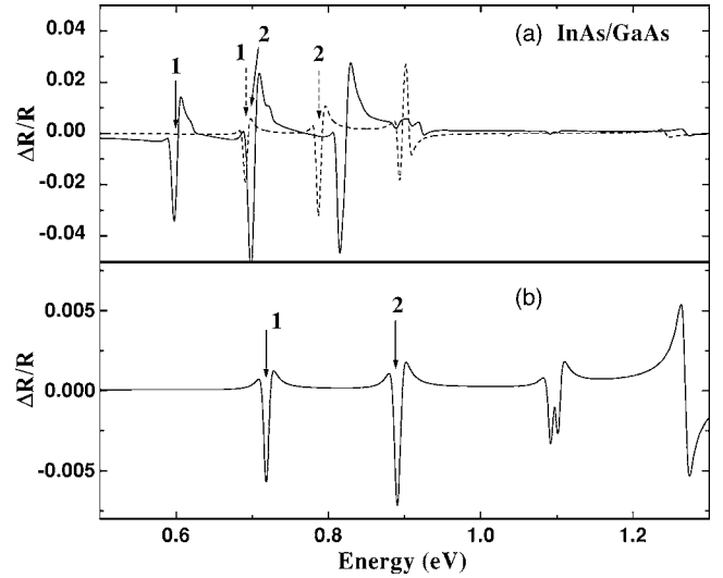
FIG. 3. Electroreflectance spectrum for InAs quantum lenses. Solid lines correspond to the lens domain a = 16 nm, b = 14.56 nm and dashed lines to a = 20.5 nm, b = 10.46 nm. Optical configurations (a) \kappa \parallel \mathbf{F} \parallel \hat{\mathbf{z}} and \hat{\mathbf{e}} \perp \hat{\mathbf{z}} . (b) \kappa \perp \mathbf{F} \parallel \hat{\mathbf{z}} and \hat{\mathbf{e}} \parallel \hat{\mathbf{z}} . In the calculation a value of F = 50 kV/cm is used. Allowed excitonic optical transitions are indicated by arrows
