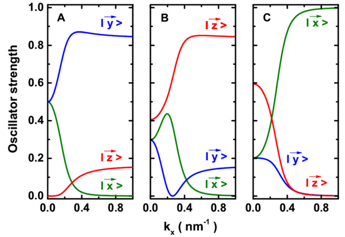
FIG. 5. Triptych representation of the expansion of A (left), B (middle), and C (right) levels against k_x . At high values of k_x , the ground state valence band (A) is dominantly built from |\vec{y}\rangle Bloch state and from about 15 percents |\vec{z}\rangle state. The second level (B) is dominantly built from |\vec{z}\rangle Bloch state and from about 15 percents |\vec{y}\rangle state. Note the quasi similar expansion of A and B through |\vec{y}\rangle and |\vec{z}\rangle , respectively. Last for high values of k_x , it appears the C is built of |\vec{x}\rangle Bloch state only. These expansions impact the selection rules for band to band transitions.
