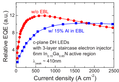
FIG. 10. (Color online) Relative EQE of two c -plane LEDs with SEI inserted under the active region: one with and one without EBLs. The LEDs were measured under pulsed current with 1 \mu s pulse width and 0.1% duty cycle. The SEI includes three intermediate InGaN layers with In compositions of 3%, 6%, and 10%, in the given order.
