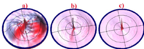
FIG. 2. (Color online) Comparison of (006) pole figures of \text{BaO}(\text{Fe}_2\text{O}_3)_6 films: (a) thicker films deposited on GaN. (b) 250 nm thick films deposited at 880^\circ\text{C} on GaN, and (c) 250 nm thick films deposited at 880^\circ\text{C} with a 25 nm MgO buffer layer on GaN.
