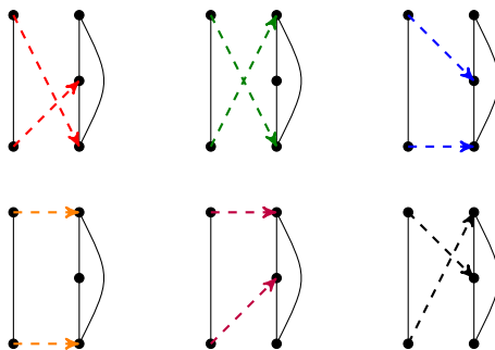
Figure 1.10: All homomorphisms from K_2 to K_3
