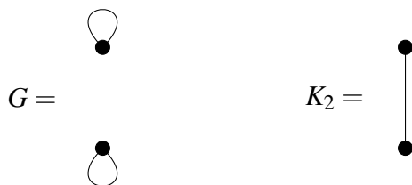
Figure 3.1: Nonisomorphic graphs G and K_2 .
