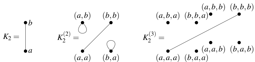
Figure 2.1: The complete graph on two vertices, K_2 , the second inner power, K_2^{(2)} , and the third inner power, K_2^{(3)} .
