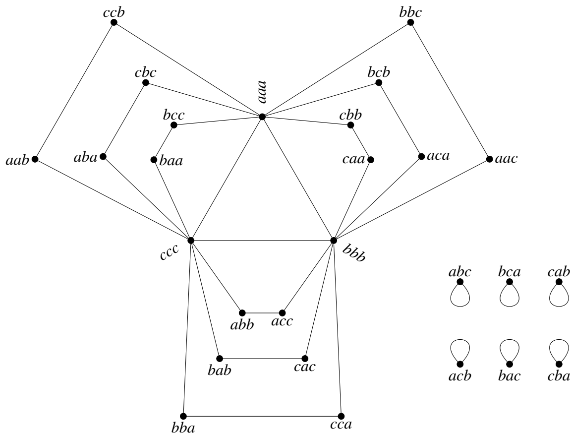
Figure 2.2: The third inner power, K_3^{(3)} , of K_3 . For convenience, the vertices are labeled without parentheses or commas. Hence abb = (a, b, b) .
