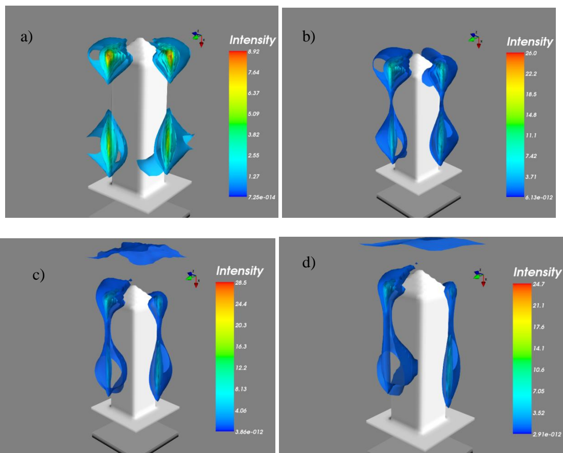
Figure 13: Localization dependent on incidence angle, with 30 nm silver thin film, 572 nm wavelength, 45^\circ linearly-polarized light. a) Normal incident light, b) 30^\circ incident light, c) 45^\circ incident light, d) 60^\circ incident light
