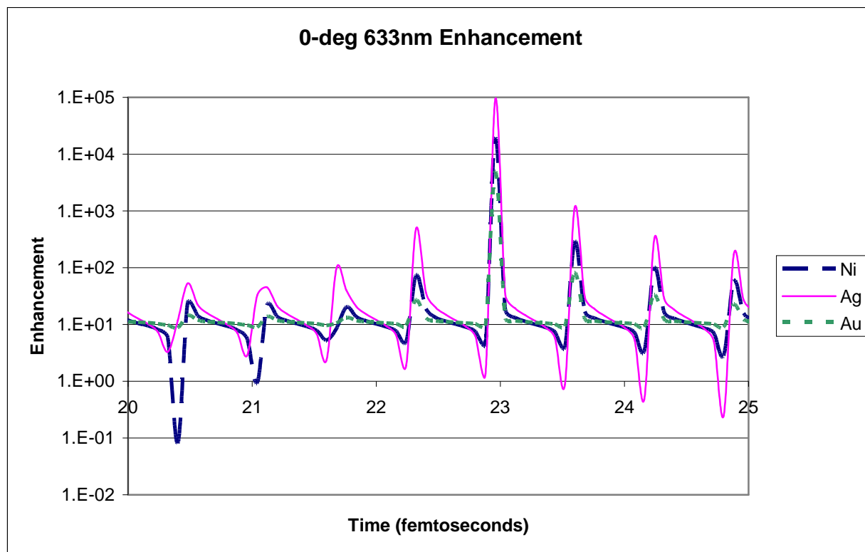
Figure 18: Enhancement with normal-incident, 45° linearly-polarized light with 633 nm wavelength at the apex corner between 20 and 25 fs.
