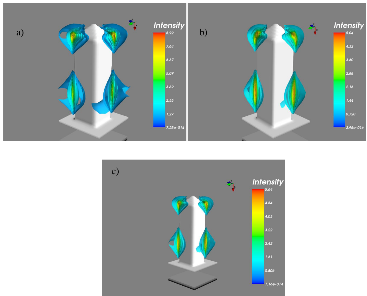
Figure 11: Light localization dependent on 30 nm metal film, with 572 nm normal incidence light, 45^\circ linearly polarized. a) silver, b) gold, c) nickel.
