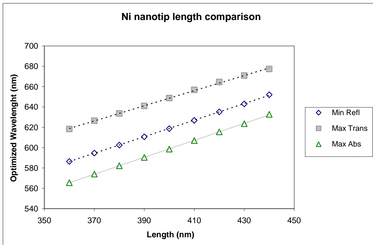
Figure 7: Optimized wavelengths for varying nanotip length.
