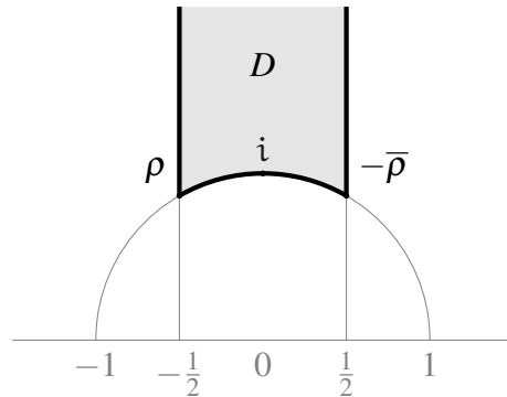
Figure 2.1: The fundamental domain D of \mathrm{PSL}_2(\mathbb{Z}) .
