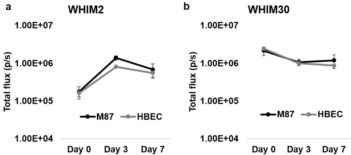
Figure 2.2: WHIM2 and WHIM30 cell viability in suspension culture over time. Viability of WHIM2 ( a ) and WHIM30 ( b ) cells cultured in suspension in two different media (M87, HBEC) immediately after plating (day 0), and after 3 and 7 days in culture. These graphs represent one of two independent experiments per PDX line, the others of which are shown in Fig. 2.1. Graphs are shown in log 10 scale. Error bars represent standard deviation of triplicate values for each condition. Reprinted by permission from Springer Nature: [149] © Springer Science+Business Media, LLC (2018)
