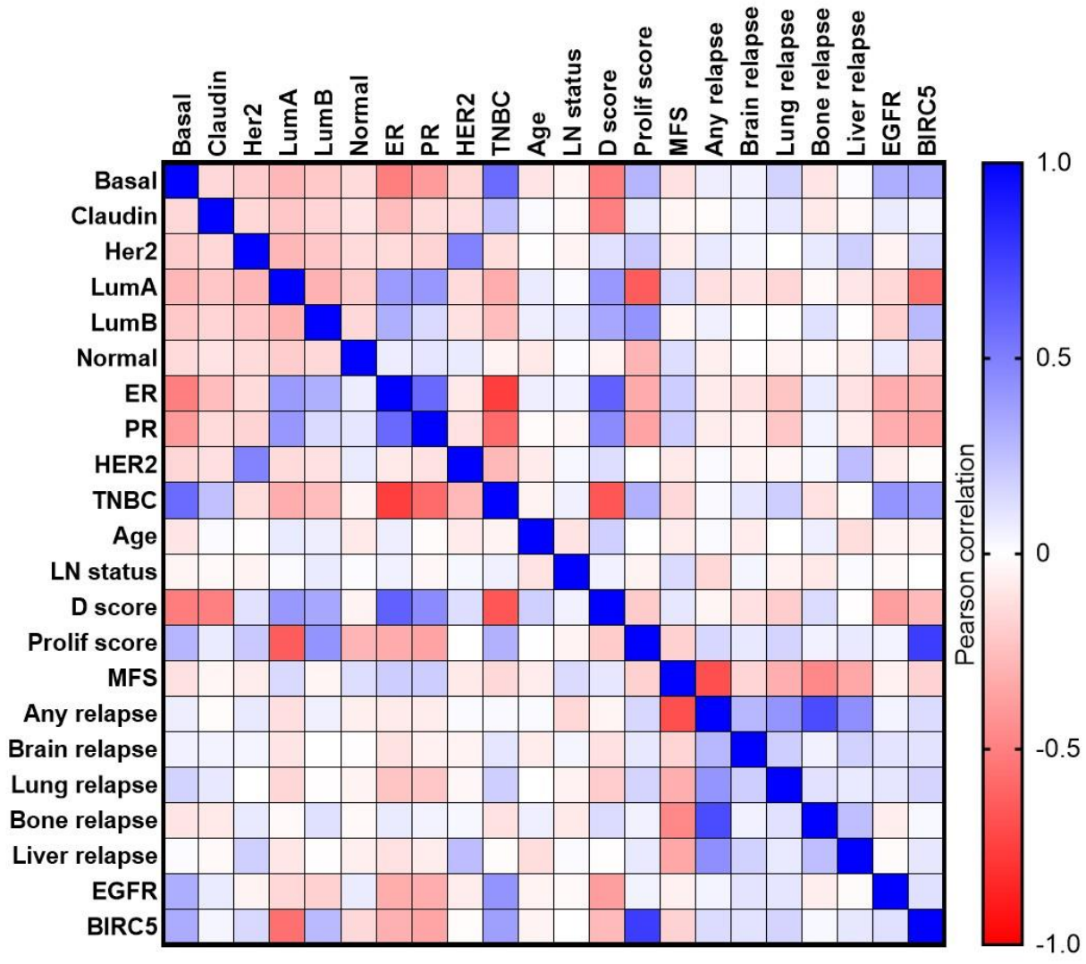
Figure 3.11: EGFR and BIRC5 expression correlate with clinical characteristics of patient tumors. Using an 855-patient dataset consisting of gene expression data as well as clinical information, Pearson correlations were performed to assess the relationships of EGFR and BIRC5 expression with clinical parameters. Intrinsic subtype: basal-like (Basal), claudin-low (Claudin), luminal A (LumA), luminal B (LumB), HER2-enriched (Her2), normal-like (Normal). Receptor status: estrogen receptor (ER), progesterone receptor (PR), human epidermal growth factor receptor 2 (HER2), triple-negative breast cancer (TNBC). Other parameters: patient age, lymph node (LN) status, differentiation (D) score, proliferation (Prolif) score. Clinical outcomes: metastasis-free survival (MFS), relapse-free survival (any relapse, brain, liver, lung, bone). Heatmap depicts Pearson correlation values for each comparison of parameters: negative correlation (red), no correlation (white), positive correlation (blue). Reprinted from [190]
