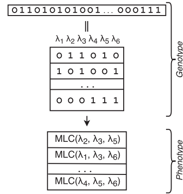
Fig. 3. Genotype and phenotype of an individual.
