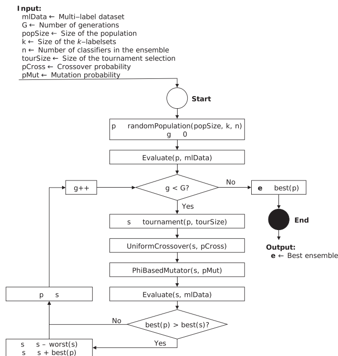
Fig. 2. Flowchart of the evolutionary process.
