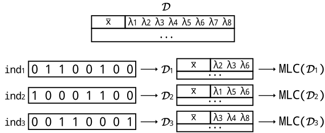
Fig. 2. Example of individuals of the evolutionary algorithm.
