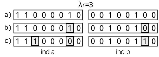
Fig. 3. Fixing the individual creation when a label cannot be shared in a_l individuals.
