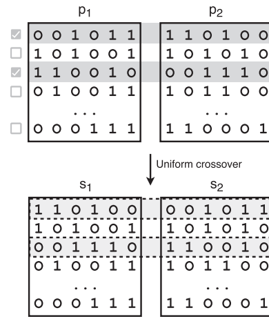
Fig. 5. Uniform crossover operator.
