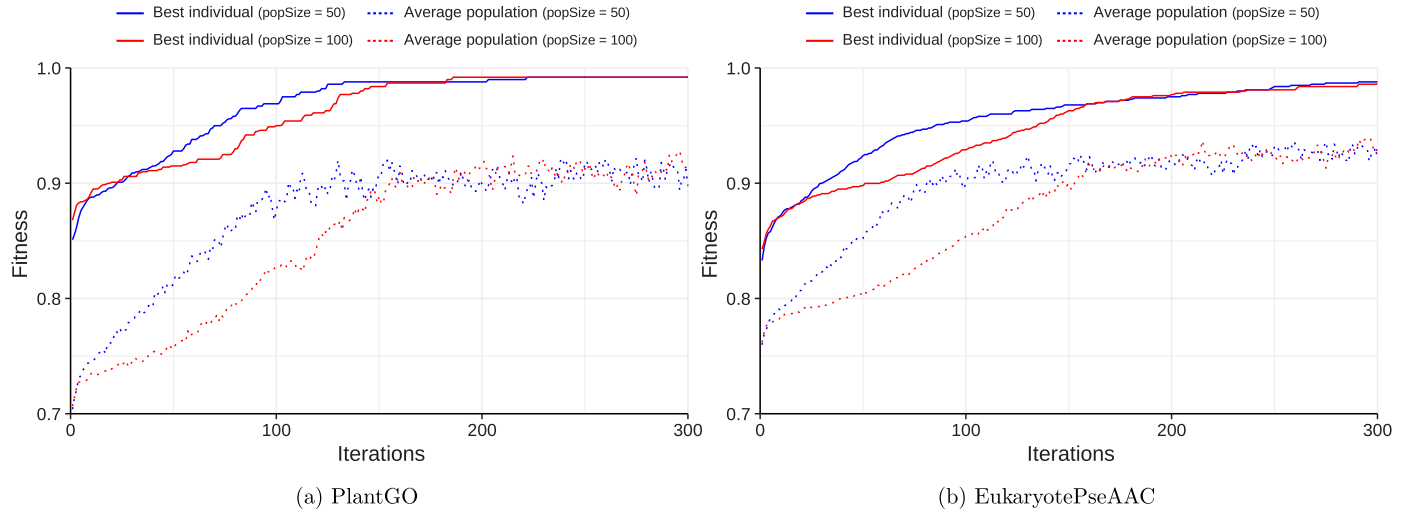
Fig. 8. Variation in fitness of the best individual and the average value of fitness of the population for PlantGO and EukaryotePseAAC datasets.
