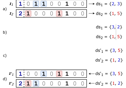
Figure 4: Example of crossover operator.
