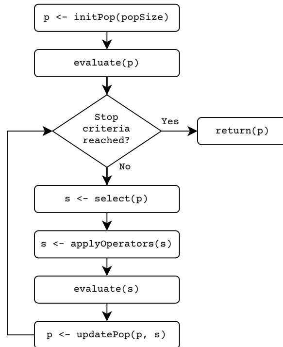
Figure 1.10: Main steps of EAs.
