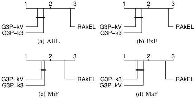
Fig. 5. Critical diagrams of Holm's test at 95% confidence for the comparison between G3P-kEMLC and RAKEL. G3P-kEMLC-3 and G3P-kEMLC-V are indicated as G3P-k3 and G3P-kV, respectively.
