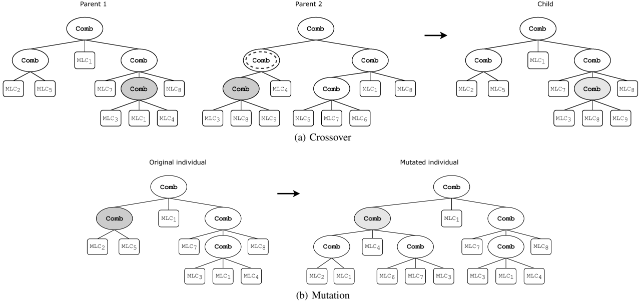
Fig. 4. Genetic operators.
