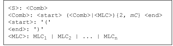
Fig. 2. Free-context grammar.
