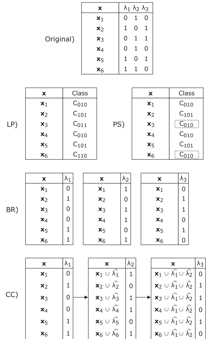
Fig. 1. Main problem transformations in MLC. For PS, labelsets appearing less than 2 times are pruned and reintroduced with most frequent subsets.
