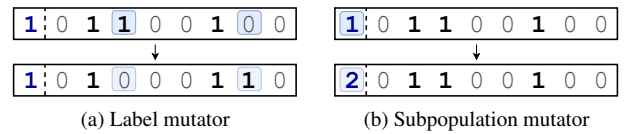
Figure 5: Mutation operators.
