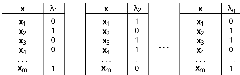
Figure 1.4: BR transformation.
