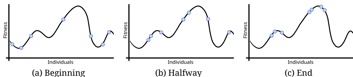
Figure 1.11: Operation of EAs along the iterations.
