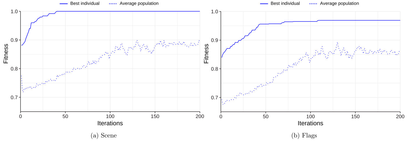
Fig. 7. Variation in fitness of the best individual and the average value of fitness of the population for Scene and Flags datasets.
