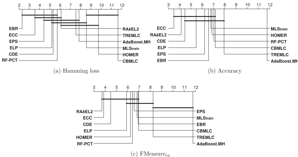
Fig. 1. Critical diagrams for the example-based metrics: results of the Shaffer’s test at 95% confidence for (a) Hamming loss, (b) accuracy and (c) FMeasure ex .
