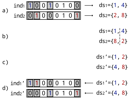
Fig. 4. Example of crossover operator.
